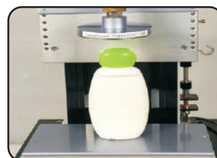
CAPPING-FORCE
