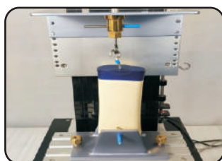
DE-CAPPING-FORCE
