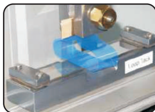
LOOP TACK
