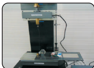
COF-ON-UTM
