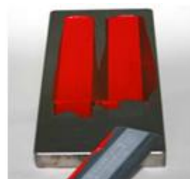
HEGMAN GAUGE (GRINDING GAUGE)
