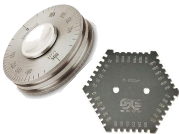
W F T GAUGE (WHEEL / COMB)
